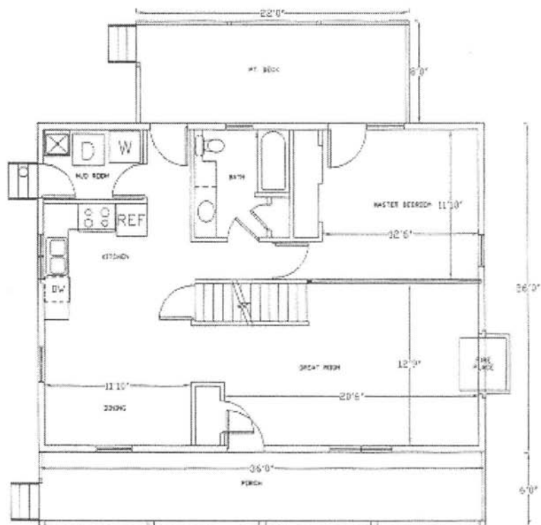
1st FLOOR
