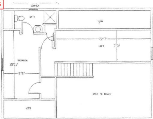
2nd FLOOR
